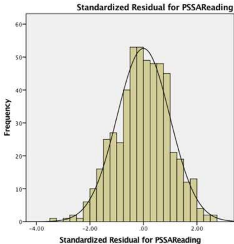
Figure 1. Histogram of standardized residuals for PSSA reading scores
