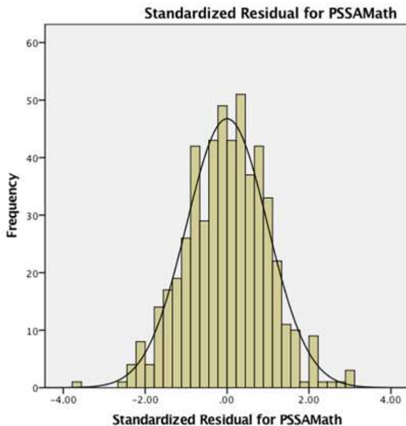
Figure 2. Histogram of standardized residuals for PSSA math scores
